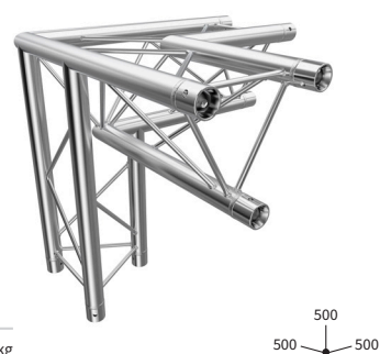
3-WEG ECKE | 3-WAY CORNER C34 CODE F23C34
