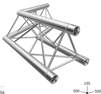
120° ECKE | CORNER C22 CODE F23C22
