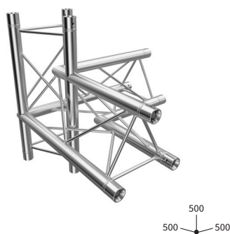
4-WEG ECKE | 4-WAY CORNER C44 CODE F23C44
