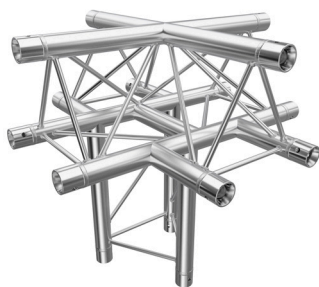
5-WEG ECKE | 5-WAY CORNER C52 CODE F23C52
