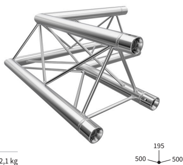
90° ECKE | CORNER C21 CODE F23C21
