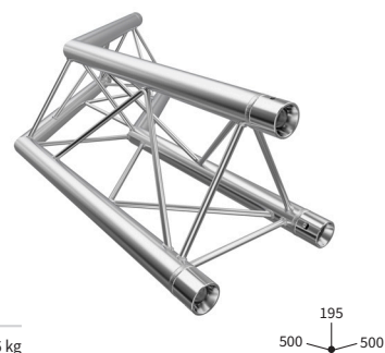
135° ECKE | CORNER C23 CODE F23C23
