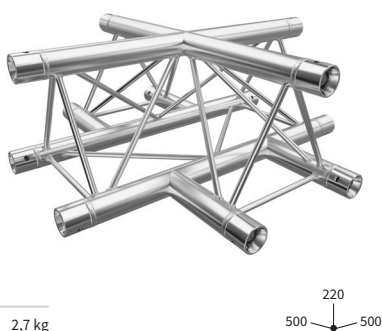
4-WEG ECKE | 4-WAY CORNER C41 CODE F23C41
