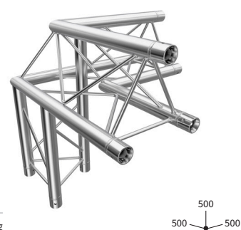
3-WEG ECKE | 3-WAY CORNER C31 CODE F23C31
