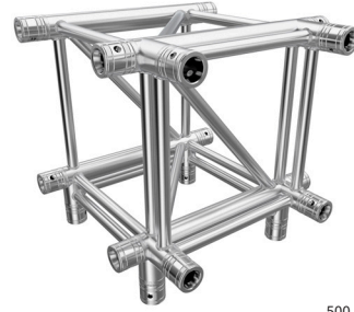
T-STÜCK | JOINT T40 P CODE F44T40P
