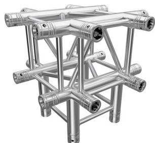
X-STÜCK | JOINT C55 CODE F34C55
