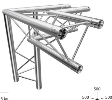
3-WEG ECKE | 3-WAY CORNER C33 CODE F23C33
