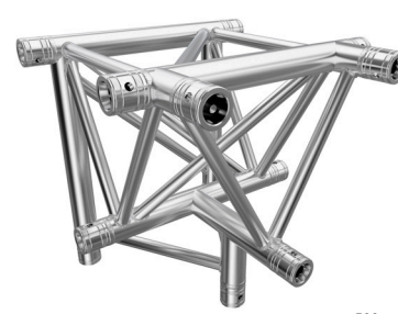
T-STÜCK | JOINT T42 CODE F43T42
